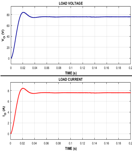
Figure 14: Voltage across Load and Current through Load for converter operation in buck-boost mode ( T_{ON}>0.5T_s )
