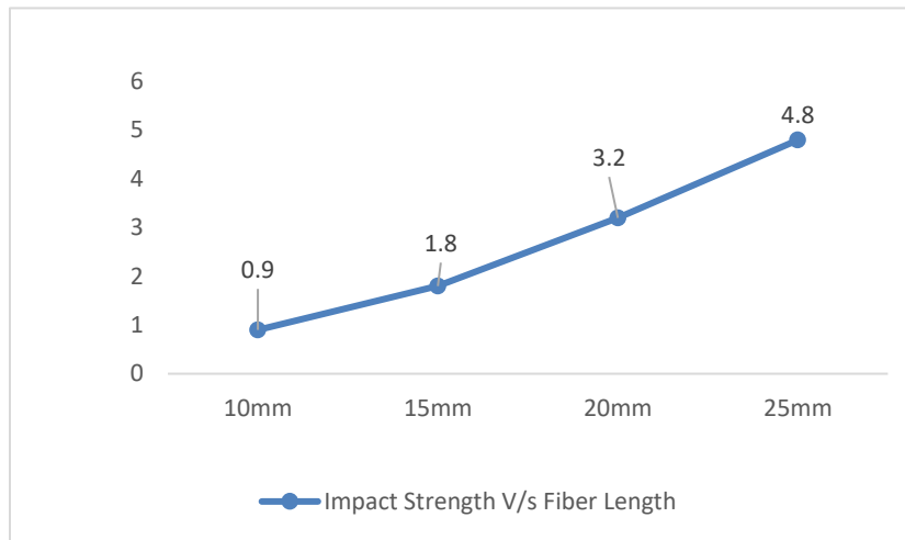
Figure 6. Graph between Impact strength and fiber length.
