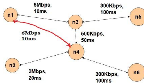
Fig.4. Creates new path with help of ADC
