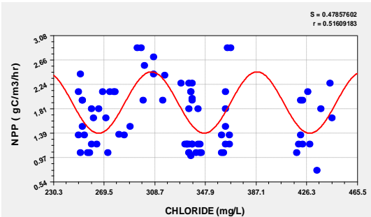
Fig.8. Sinusoidal fit showing the mathematical relationship between Chloride and NPP.
