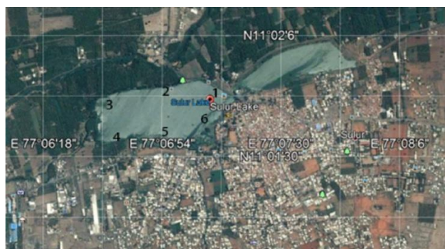
Fig.1. Satellite view of Sulur Lake showing the location of six sampling sites.
