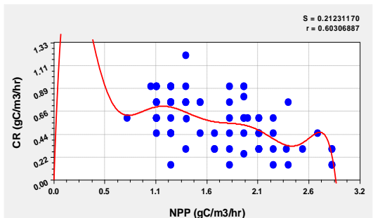
Fig.11. Polynomial fit showing the mathematical relationship between NPP and CR.
