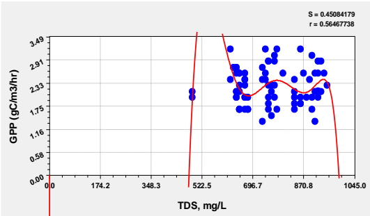
Fig.7. Polynomial fit showing the mathematical relationship between TDS and GPP.
