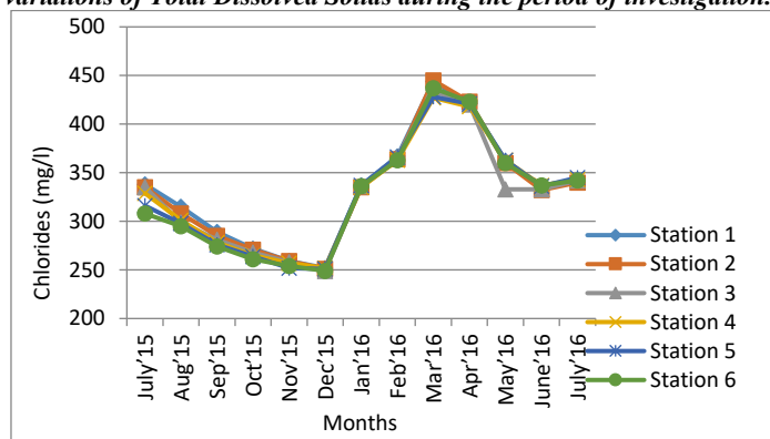
Fig. 5. Seasonal variations of Chlorides during the period of investigation. (July'15-July-16).
