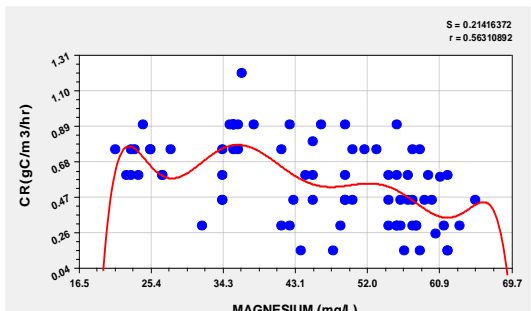
Fig.10. Polynomial fit showing the mathematical relationship between Magnesium and CR.
